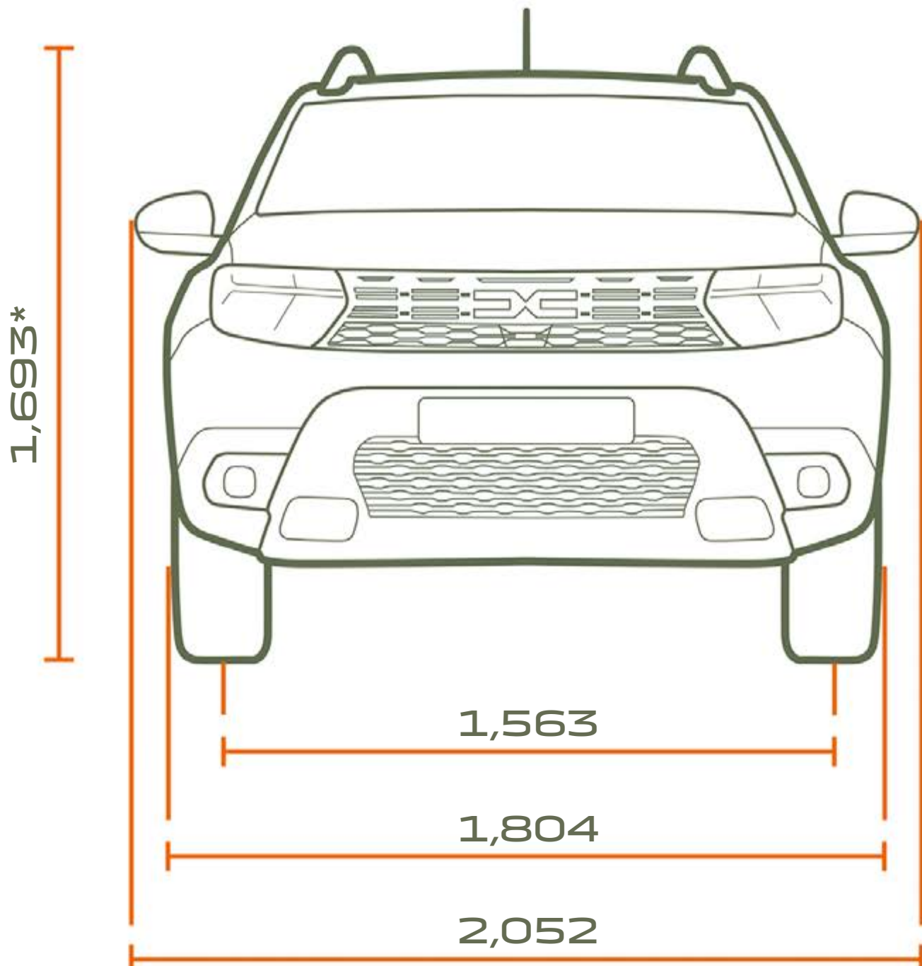
FRONT VIEW
